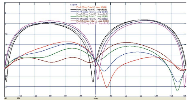
Typical elevation cuts at 466 MHz
